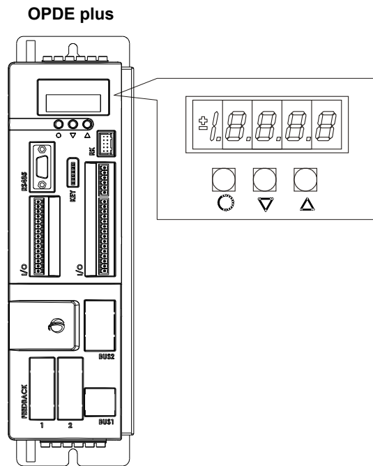
FIG. 1 (Physical disposition)
