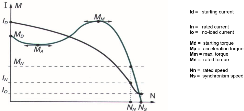
3-phase induction motor torque (M) and current (I) curve according to number of revolutions (N).
