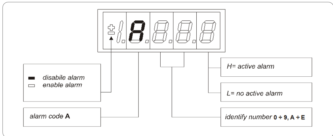
FIG. 6 (Allarms ALL)
