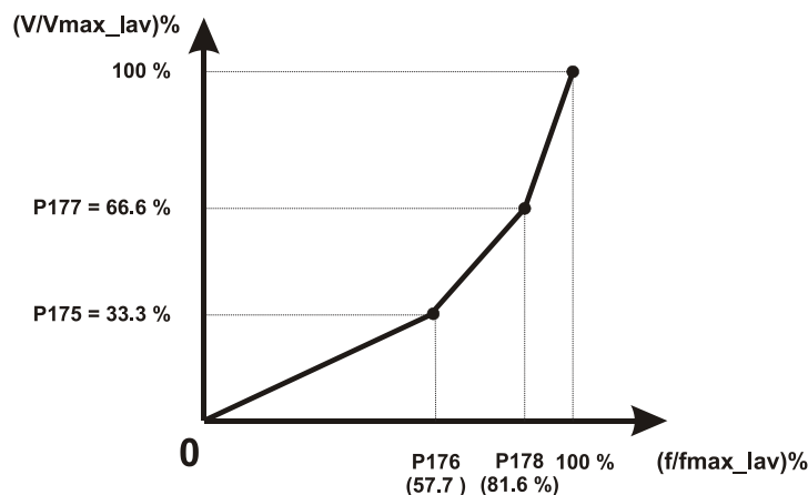
"TYPICAL CURVE WITH QUADRATIC TORQUE LOAD"
